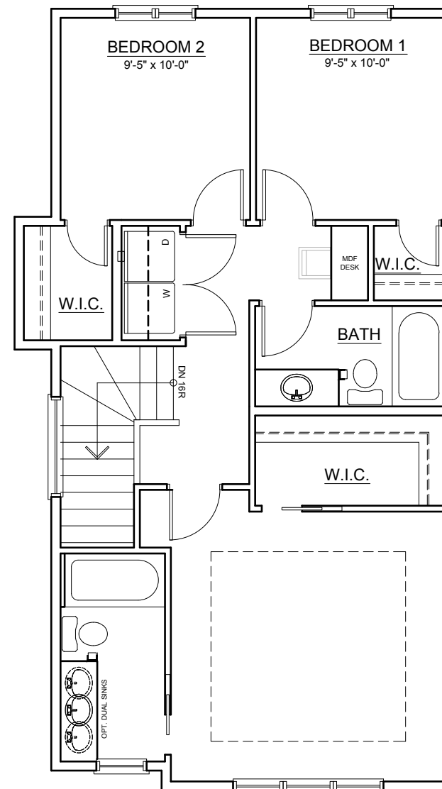
UPPER FLOOR ± 785 SQ. FT.
