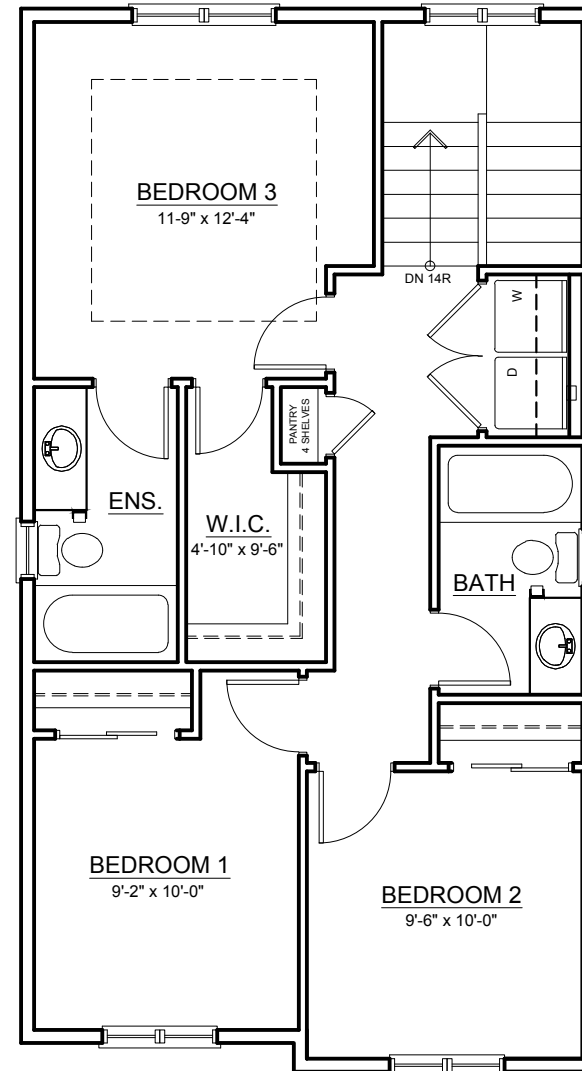
UPPER FLOOR ± 731 SQ. FT.
